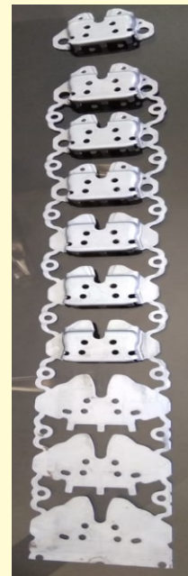
Car Part With Progressive Tools 28000 Pcs / 8 Hrs For Suzuki Car
