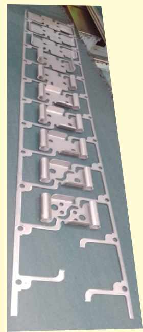
Car Door Hinge With Progressive Tools 56000 Pcs / 8 Hrs For GTIP
