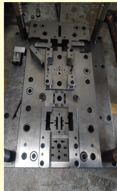
Progressive Tools For Car parts 28000 Pcs / 8 Hrs
