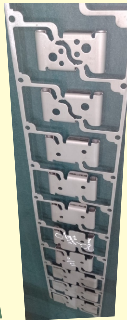
Car Door Hinge With Progressive Tools 56000 Pcs / 8 Hrs For GTIP
