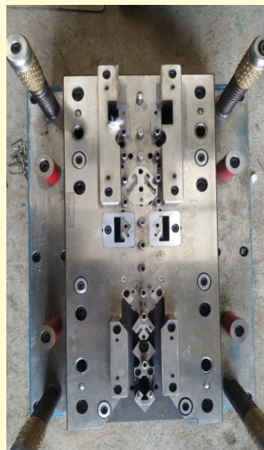
Progressive Tools For Car parts 28000 Pcs / 8 Hrs
