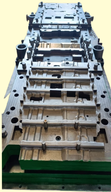
Progressive Tools For Car parts 28000 Pcs / 8 Hrs HSLA 540
